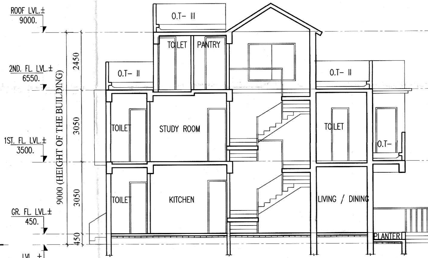
SECTION AT E-E
