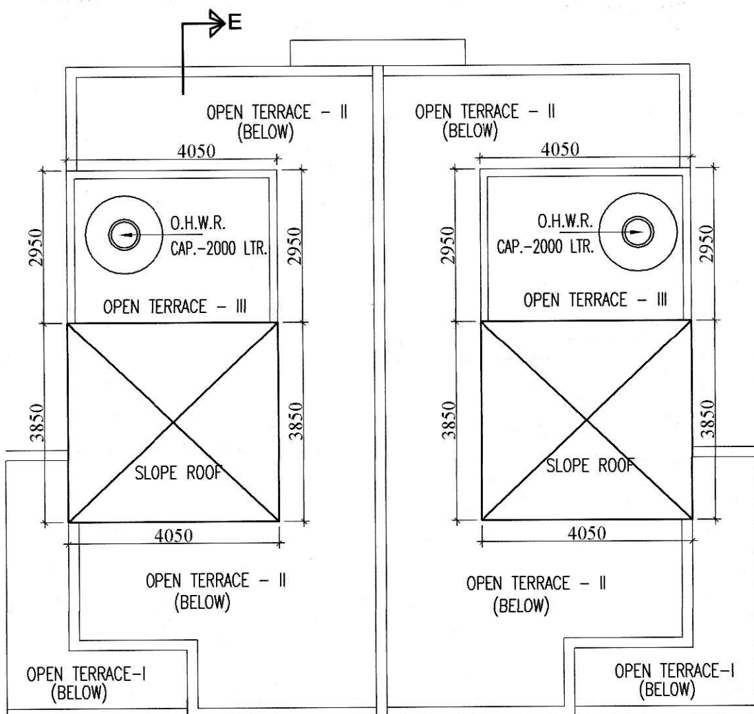
ROOF PLAN
